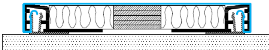
Plywood Insert For Artwork/Signage
