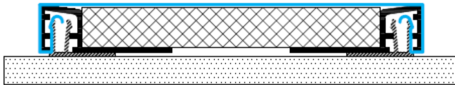
Tackable 24 LB Density Mineral Fiberboard (Micore)
